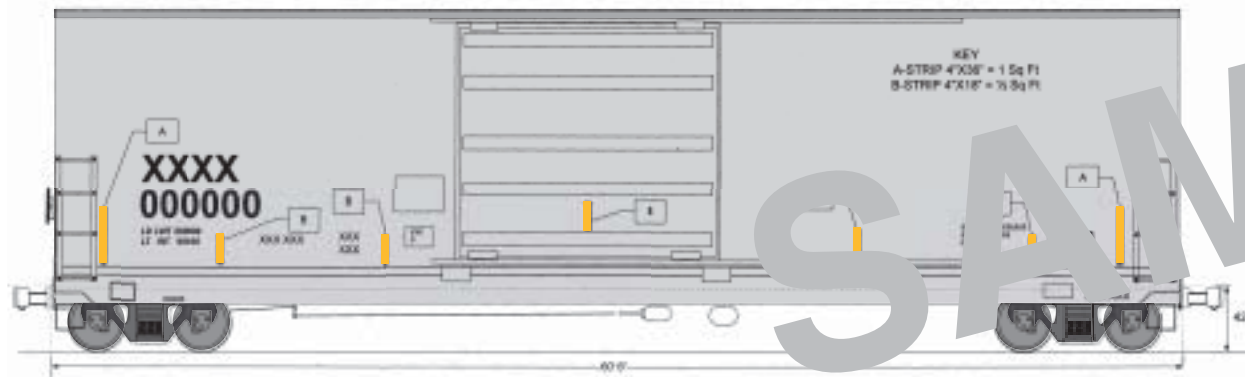
Figure 1 Yellow vertical reflective sheeting (4.5 sq. ft.) pattern applied to a typical 60' 6" Box Car.
